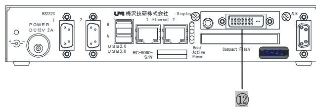
RC-9060-DVI+AUDIO TypeW10
